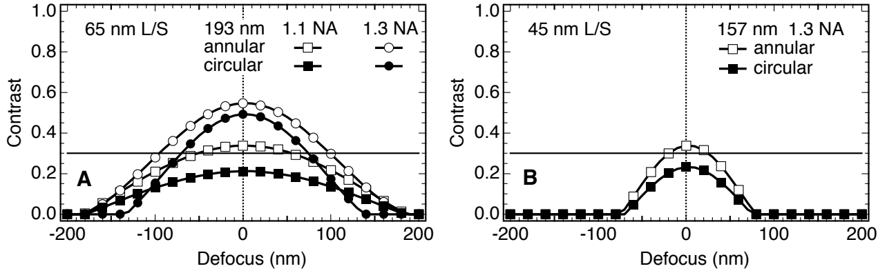
Figure 4. Comparison of contrast vs. focus for annular ( \sigma_{in} = 0.4 , \sigma_{out} = 0.6 ) and circular ( \sigma = 0.6 ) illumination. (a) 65 nm L/S, \lambda = 193 nm; (b) 45 nm L/S, \lambda = 157 nm.
