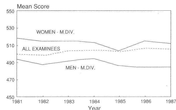
GRE Verbal Scores of Prospective M.Div. Students
