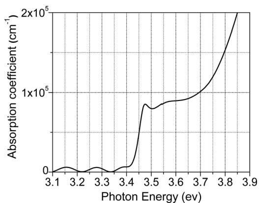
FIG. 2. Absorption spectrum of the epitaxial material used to fabricate the devices of Fig. 1.
