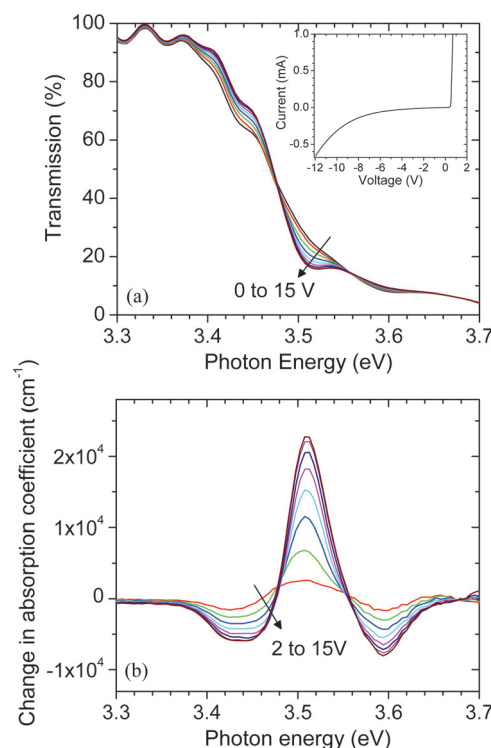
FIG. 5. (Color online) (a) Normalized transmission spectra through a GaN/AlGa \text{N} multiple-QW modulator for different values of the applied reverse bias voltage (0, 2, 4, 6, 8, 10, 12, 14, and 15 V). The inset shows the current-voltage characteristics of the same device. (b) Differential absorption spectra derived from the traces of (a).
