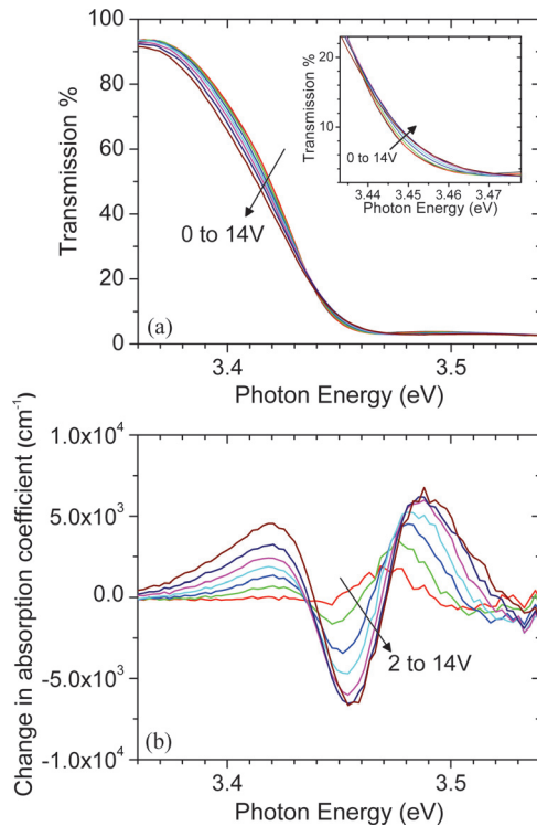
FIG. 3. (Color online) (a) Normalized transmission spectra through a bulk GaN modulator for different values of the applied reverse bias voltage from 0 to 14 V in steps of 2 V. The inset shows a zoom-in of these traces near the excitonic resonance. (b) Differential absorption spectra derived from the traces of (a).
