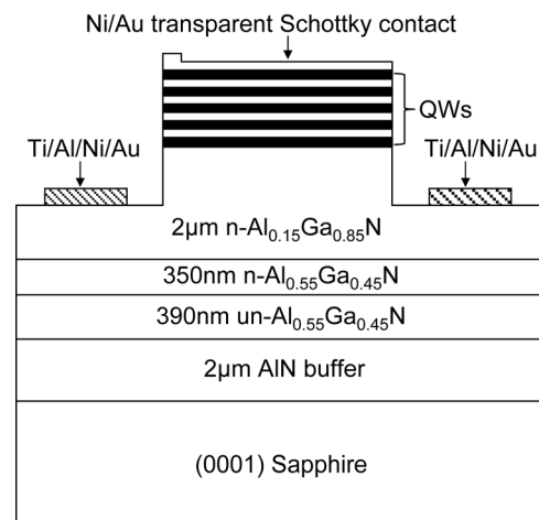
FIG. 4. Schematic cross-sectional view of a GaN/AlGaN multiple-QW electroabsorption modulator developed in this work.
