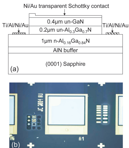
FIG. 1. (Color online) (a) Schematic cross-sectional view of the bulk GaN electroabsorption modulators developed in this work. (b) Top-view micrograph of a fabricated device.
