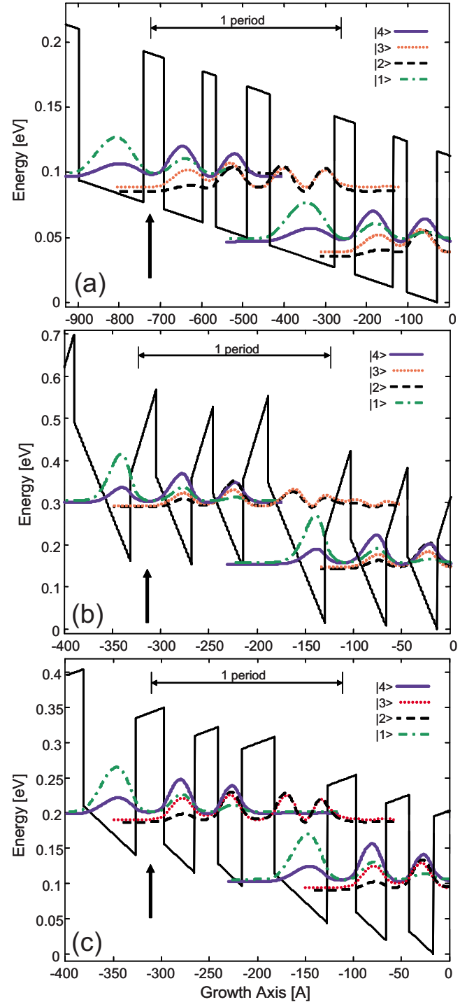
FIG. 2. (Color online) Conduction-band profile and squared envelope functions of (a) the GaAs/Al 0.15 Ga 0.85 As, (b) the GaN/Al 0.15 Ga 0.85 N, and (c) the ZnO/Mg 0.15 Zn 0.85 O QC gain media considered in this study.
