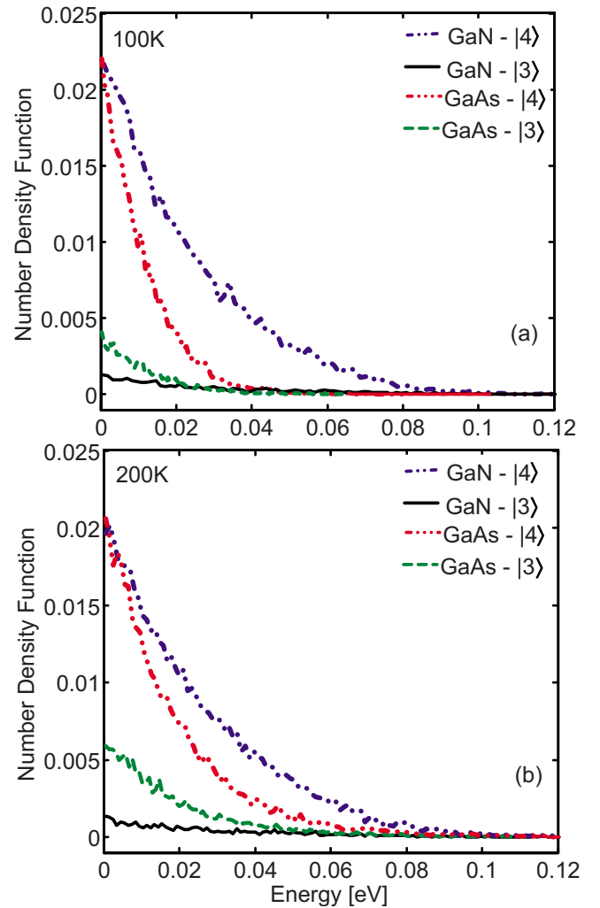
FIG. 5. (Color online) Calculated NDF of the upper |4\rangle and lower |3\rangle laser states of the GaAs and GaN structures at temperatures of 100 K (a) and 200 K (b).
