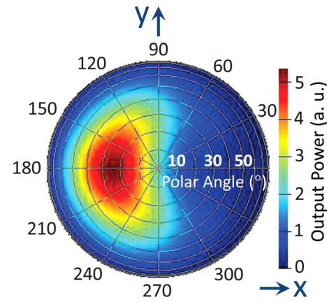
FIG. 3. Far-field radiation pattern in the array substrate produced by an electron traveling in the x direction, for \Lambda = 100 nm and d = 1 \mu\text{m} . The x - y coordinate system is the same as in Fig. 1(b).
