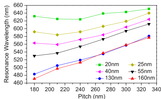
FIG. 3. (Color online) Measured plasmonic resonance wavelengths plotted vs array pitch for different NP heights (indicated in the legend).
