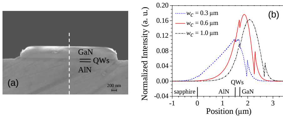
Fig. 1. (a). SEM image of the facet of a GaN/AlN QW waveguide. (b) Intensity profile of the fundamental TM mode along the dashed line of (a), for different thicknesses of the GaN cap.
