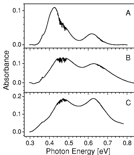
FIG. 4. Measured ISB absorbance spectra of samples A, B, and C.
