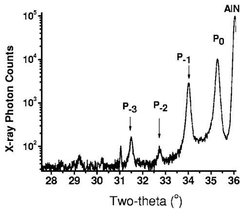
FIG. 2. On-axis \theta - 2\theta x-ray diffraction scan of sample C.
