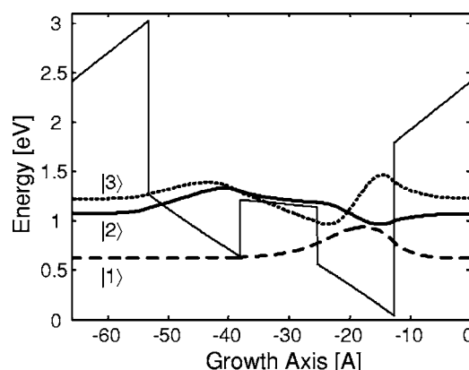
FIG. 1. Calculated conduction-band lineup and envelope functions of the three lowest bound states (referenced to their respective energy levels) of an AlN/GaN/AlGaIn CQW structure, corresponding to sample A of Table I.
