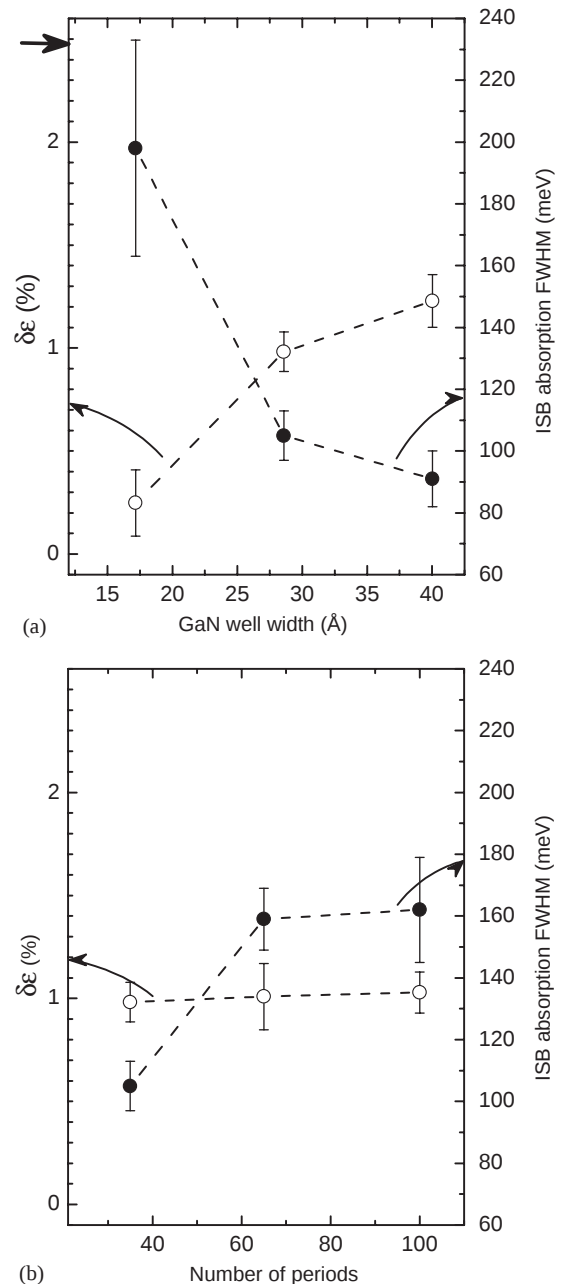
Fig. 3. (a) Variation of MQW strain relaxation with respect to AlN and corresponding ISB absorption FWHM as functions of the GaN well width (the arrow at 2.47% on the upper left-hand ordinate indicates the position of fully relaxed GaN on AlN) and (b) variation of MQW strain relaxation with respect to AlN and corresponding ISB absorption FWHM as functions of the number of periods.
