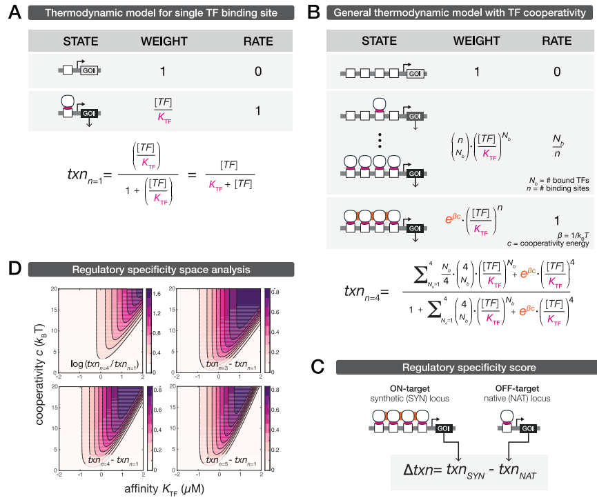
Figure S2. Description and analysis of thermodynamic model for cooperative-assembly-driven specificity, related to Figure 2
