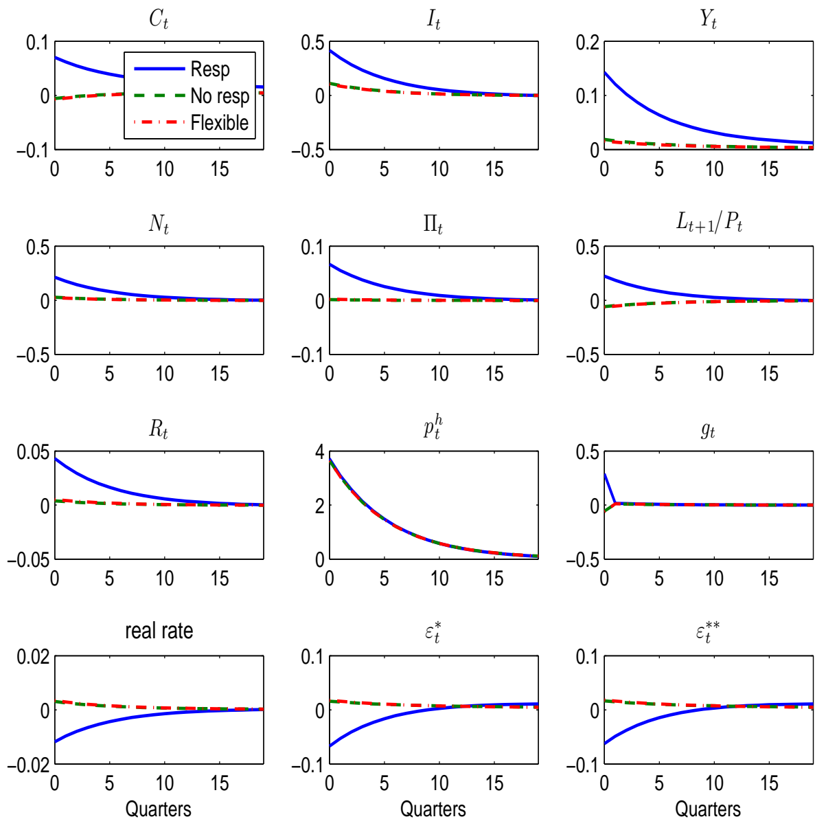
Figure 6: Impulse responses to a positive standard deviation (0.613%) sentiment shock under the interest rate rule in (42). All vertical axes are measured in percentage. The solid lines represent the case with the optimal weight on asset bubbles given in Table 1. The dashed lines represent the case with \phi_p = 0 . The dot dashed lines represent the responses in the flexible price equilibrium
