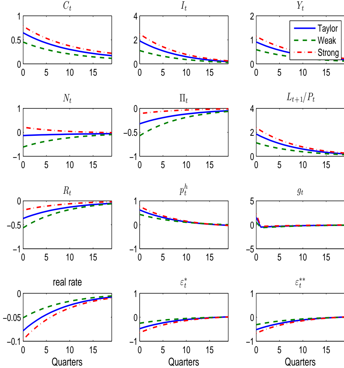
Figure 2: Impulse responses to a positive 1% technology shock. All vertical axes are measured in percentage. The solid, dashed, and dot dashed lines represent responses under the Taylor rule in (42), the weak inflation targeting rule in (43) with \phi_\pi = 1.1 , and the strong inflation targeting rule in (43) with \phi_\pi = 2 . In all these rules, \phi_p = 0 .
