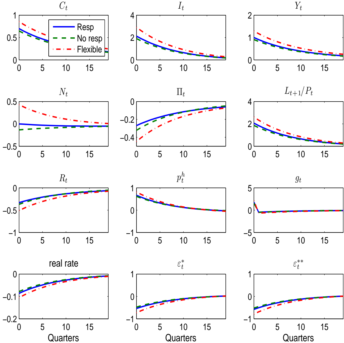
Figure 5: Impulse responses to a positive 1% TFP shock under the interest rate rule in (42). All vertical axes are measured in percentage. The solid lines represent the case with the optimal weight on asset bubbles given in Table 1. The dashed lines represent the case with \phi_p = 0 . The dot dashed lines represent the responses in the flexible price equilibrium
