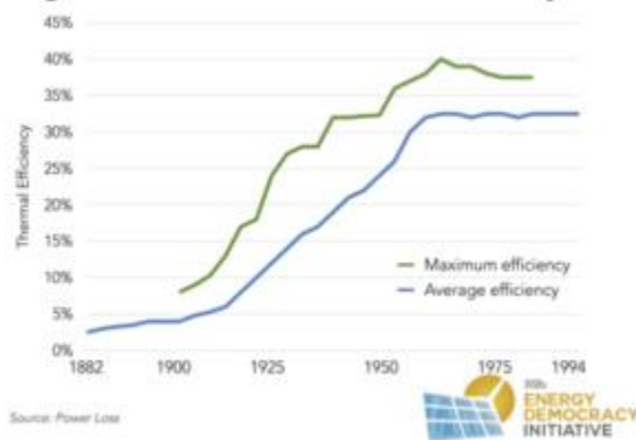
Figure 1 Power Plant Efficiency
