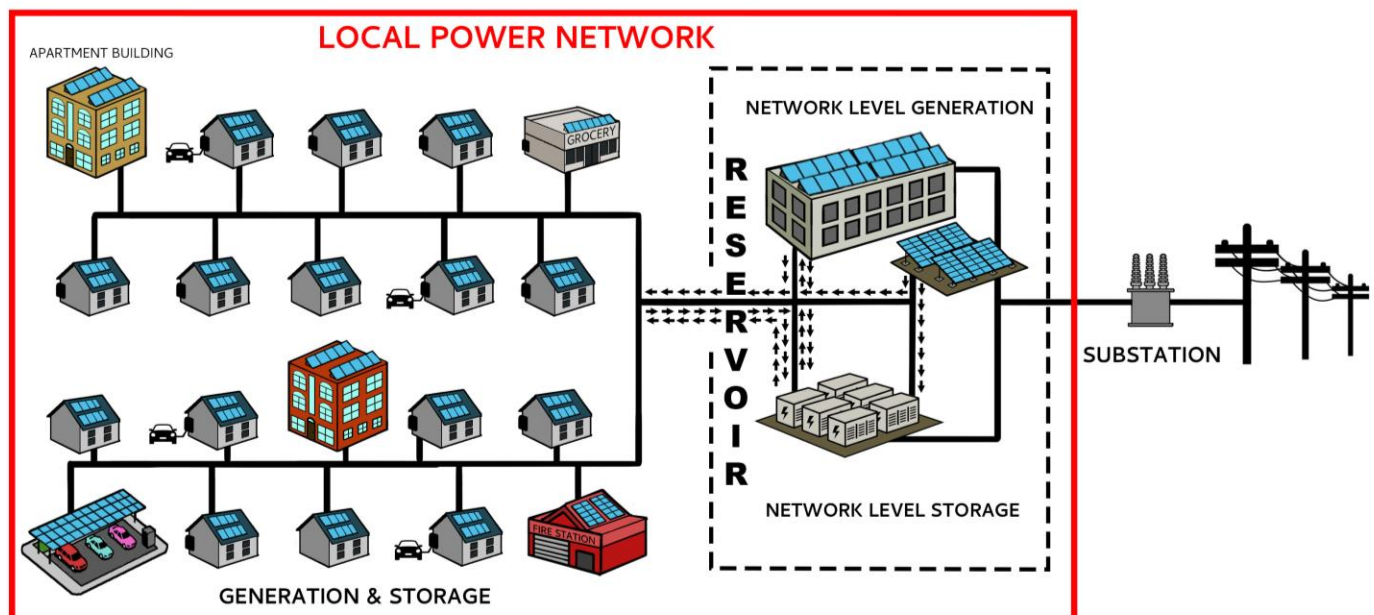
Figure 3. Schematic diagram of a Local Power Network
