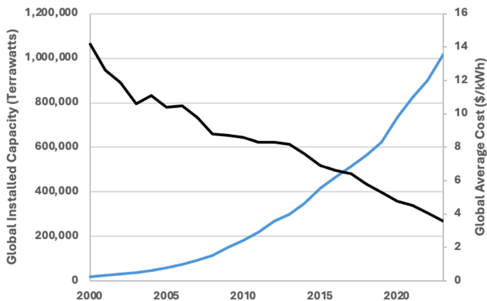
Figure 7. Global Wind Energy Installed Capacity and Average Cost, 2000–2023
