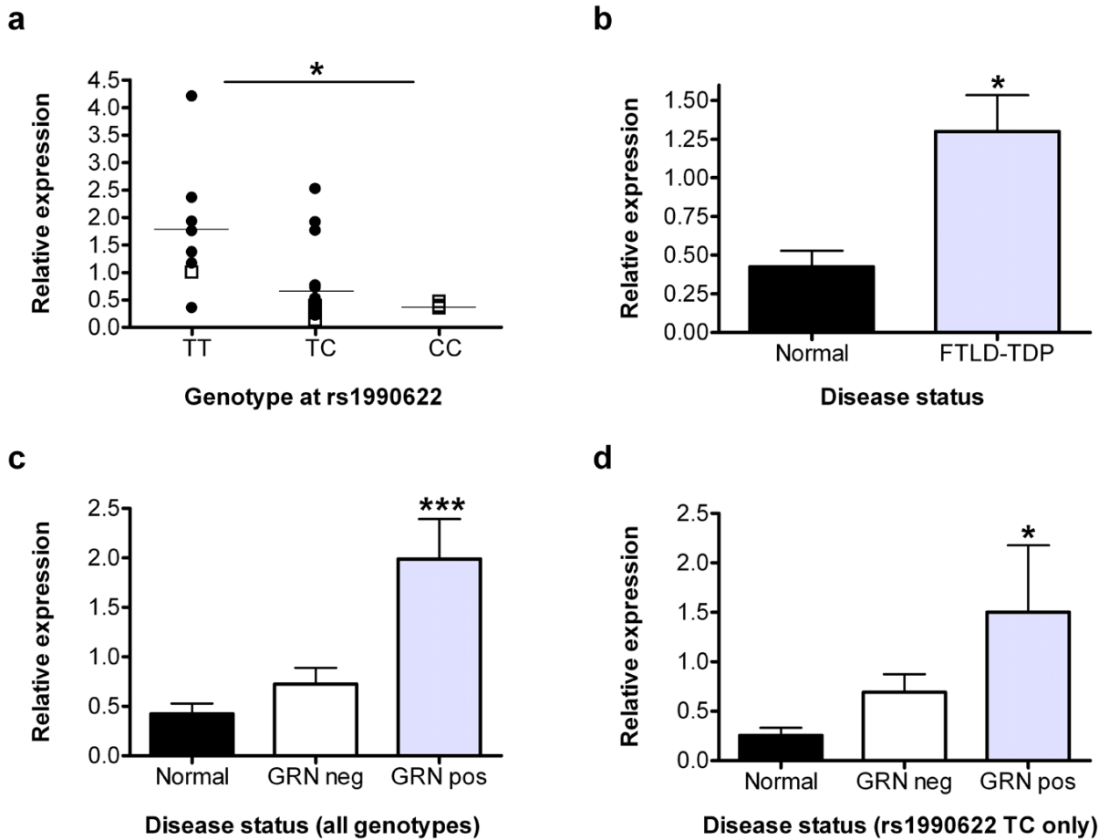
Figure 2. TMEM106B expression variation by genotype and disease state
