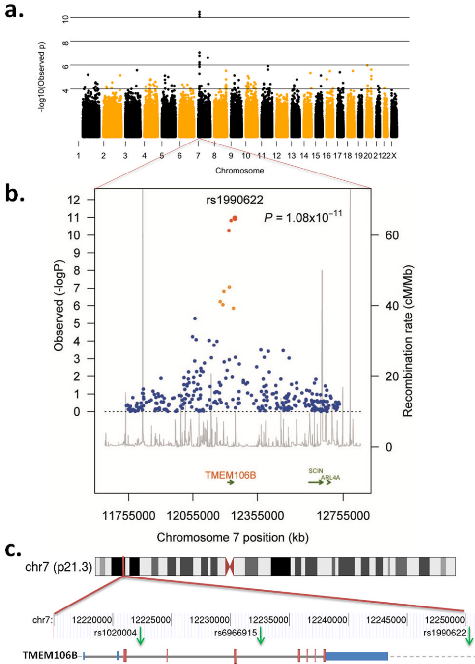
Figure 1. Region of genome-wide association at 7p21
