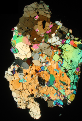
Olivine diogenite GRA 98108
