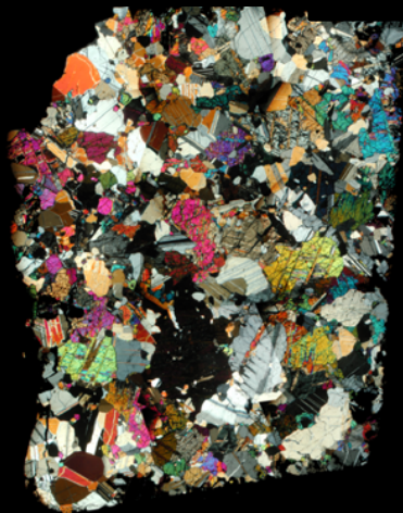
Cumulate eucrite Moore County
