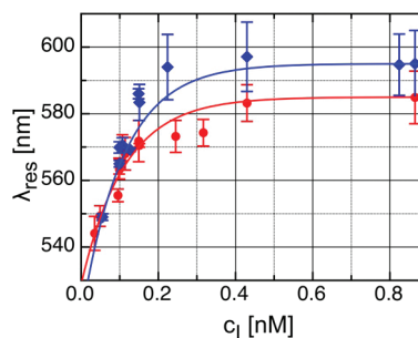
Figure 4. Resonance wavelength ( \lambda_{\text{res}} ) as function of immunolabel concentration ( c_i ) measured on dorsal cell membranes (red) and filopodia (blue). The observed red-shift as a function of increasing NP concentration indicates an increase in \rho . Exponential fits ( \lambda_{\text{res}} = \lambda_{\text{max}} - A \exp(-c_i/c_0) ) with the following parameters: \lambda_{\text{max}} = 585.0 nm; A = 56.21 nm; c_0 = 0.1124 nM (red), and \lambda_{\text{max}} = 595.0 nm; A = 76.57 nm; c_0 = 0.1079 nM (blue) are included as continuous lines to guide the eye.
