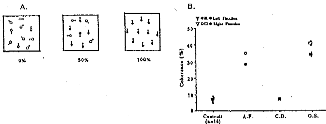
Fig. 3. Motion coherence
