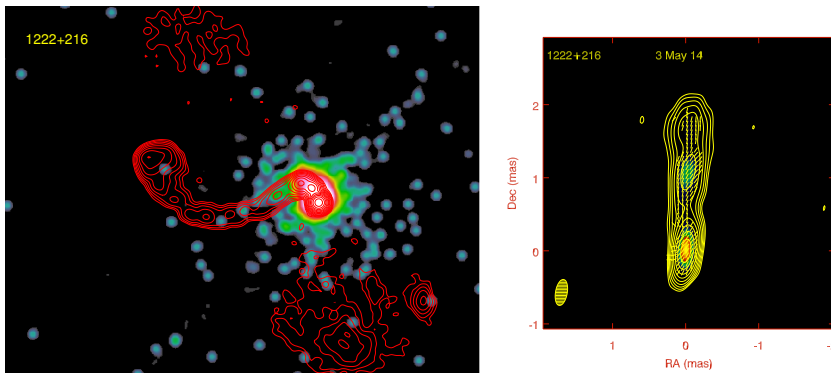
Figure 1. Left: Chandra (color scale) and VLA 5 GHz (contours) images of 4C+21.35; contours are in factors of 2 of the peak intensity of 0.93\text{ Jy/beam} . The images are convolved with a beam of \text{FWHM } 0.5 \times 0.5\text{ arcsec}^2 . Right: VLBA image of the inner jet at 43 GHz; contours are in factors of 2 of the peak intensity of 0.99\text{ Jy/beam} ; color scale corresponds to polarized intensity with peak = 62.5\text{ mJy/beam} ; line segments within the contours show direction of polarization.
