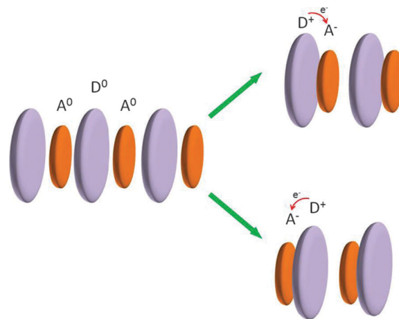
Fig. 4 Schematics of neutral-to-ionic transition in the charge transfer complex.
