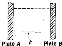
FIG. 2. Here the volume \mathcal{V} is assumed to be of a similar shape to the volume indicated in Fig. 1, but the ends of it now fall halfway between the middle of plates A and B , rather than between the middle of plates A and C .
