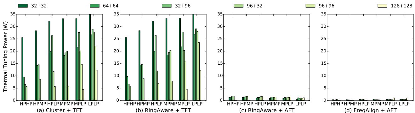
Fig. 9: Average optical tuning power when using localized tuning for Clustered , RingAware and FreqAlign workload allocation policy for 8-ary 3-stage Clos topology with U-shape layout in Figure 1(a). TFT : Target Frequency Tuning; AFT : Adaptive Frequency Tuning.
