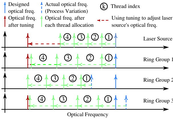
Fig. 7: Illustration of FreqAlign workload allocation policy and adaptive frequency tuning AFT policy. Every thread allocated by FreqAlign increases the temperatures of ring groups and causes a downward shift in their frequencies. When all threads are allocated, thermal tuning is used to bring all ring groups to the lowest common resonant frequency. Above, ring groups 1 and 3, as well as the laser source, are tuned to match the resonant frequency of ring group 2.
