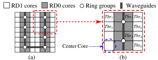
Fig. 6: (a) Classification of RD0 cores and (b) an example of RingAware allocation in a 64-core system.
