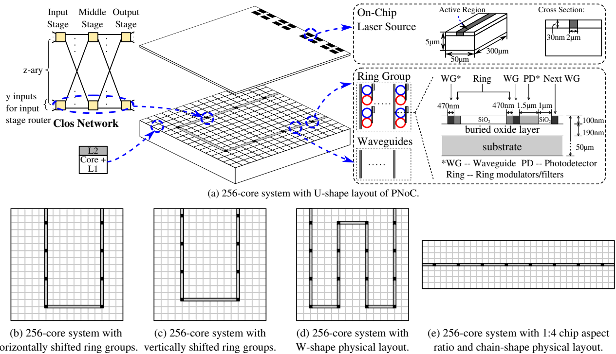
Fig. 1: Target manycore system with a PNoC (a), manycore systems with 8-ary 3-stage Clos topology and shifted physical layouts (b)-(c), and manycore systems with different logical topology and physical layout combinations (d)-(e). (d) is designed with 16-ary 3-stage Clos topology and W-shape physical layout; (e) is designed with 8-ary 3-stage Clos topology and chain-shape physical layout.
