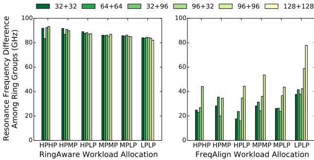
(c) Maximum process variation among ring groups. Average (maximum) power reduction is 2.04 W (3.26 W ), 60.1% (80.8%).
