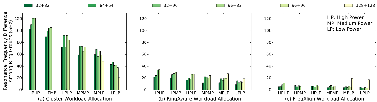
Fig. 8: Average resonant frequency differences when using Clustered , RingAware and FreqAlign workload allocation policy for U-shape layout with 8-ary 3-stage Clos topology shown in Figure 1(a). Each bar represents a workload and utilization combination case.
