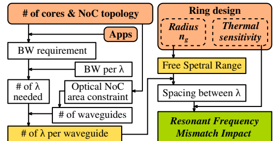
Fig. 2: PNoC design flow chart.
