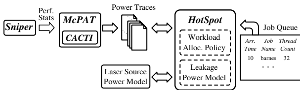
Fig. 4: Our performance [29], power [31], [30] and thermal [32] simulation setup for modeling manycore systems with a PNoC.
