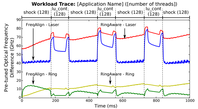
Fig. 13: Runtime optical frequency difference trace for transient case with large temporal on-chip temperature gradients prior to applying tuning methods.
