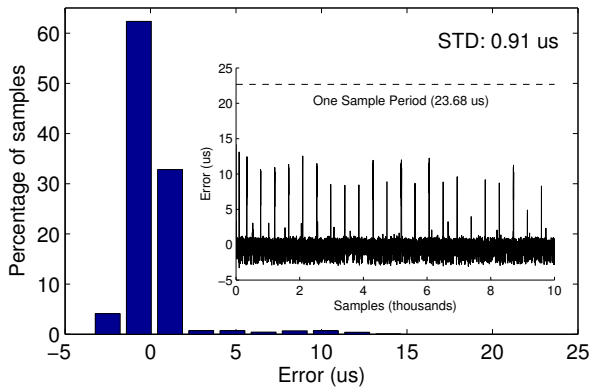
Figure 5: Histogram of the error between when a time step should have occurred and when it actually occurred. Figure inset shows a sample of the error, 95% of the error is within 1.56 \mu\text{s} .
