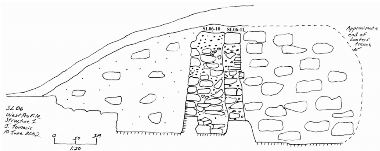
Figure 31. Western profile of southern tunnel in Str 1, Group 1, at La Sufricaya showing walls SL06-10 and SL06-11 separated by fill. Wall SL06-11 bears the mural.
