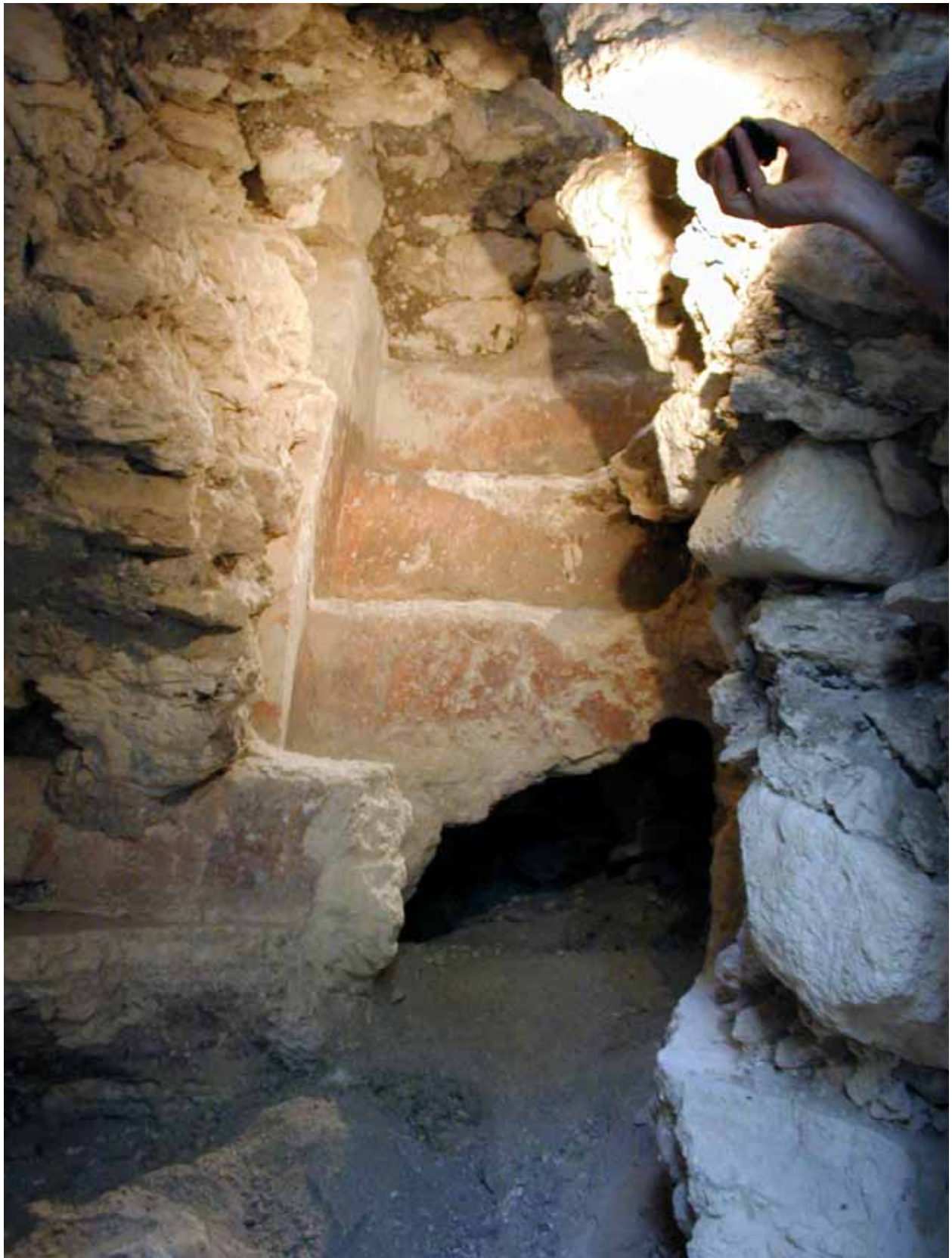
Figure 46. Phase 1 of Structure 5. Buried red painted stairway and terrace mouldings.
