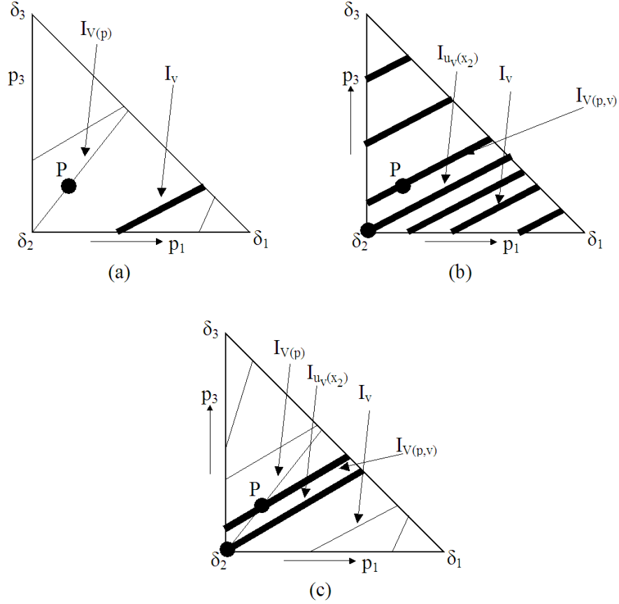
Figure 1: 1a: Fixing an indifference curve of level v . 1b: Constructing the local utility function u_v(x) . 1c: Putting them together, E_p[u(x, V(p))] = u(x_2, V(p)) , but E_p[u(x, v)] > u(x_2, v) for v \neq V(p) .
