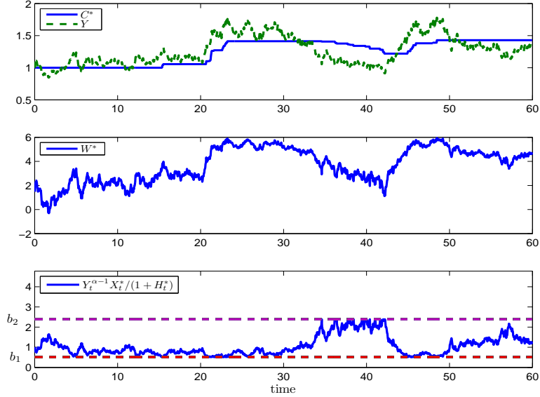
Figure 6: Simulated paths of the agent's optimal consumption C_t^* , incomes Y_t , continuation values W_t^* , and the process Y_t^{\alpha-1} X_t^*/(1+H_t^*) , t \geq 0 , for Example II. Parameter values are given by \mu = 0.02 , \sigma = 0.1 , \rho = 0.04 , and \alpha = -2 .
