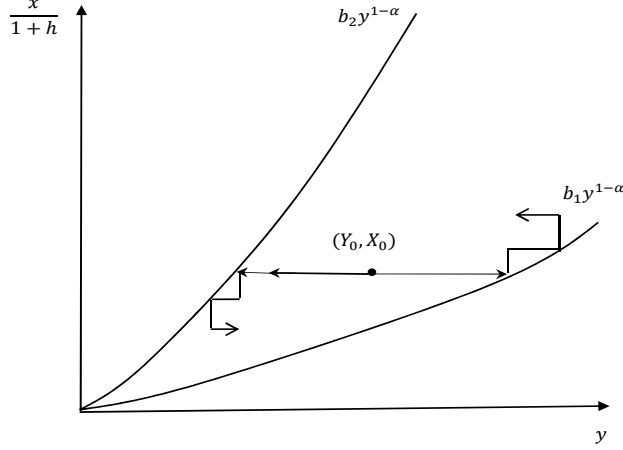
Figure 4: The state space for Example II. The two curves x/(1+h) = b_1 y^{1-\alpha} and x/(1+h) = b_2 y^{1-\alpha} partition the state space into three areas. The middle area is the no-jump region and the other two areas are the jump region.
