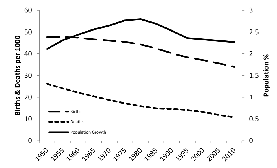
Figure 5. Africa: Crude Birth and Death Rates and Population Growth
