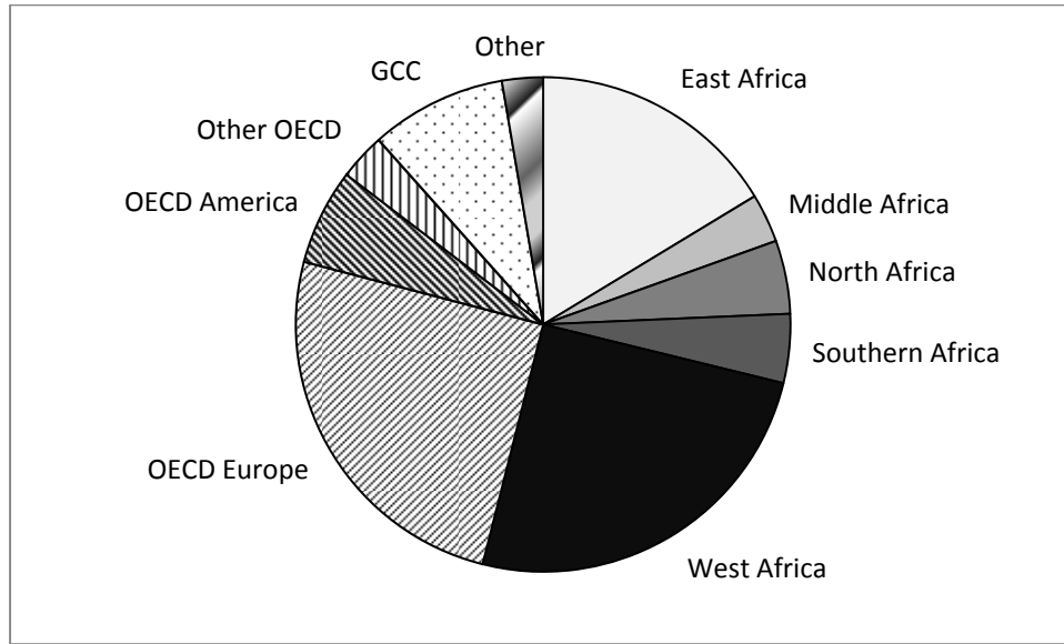
Figure 1. Location of Africa's Diaspora
