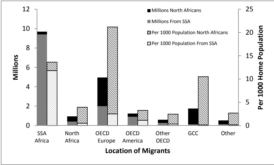
Figure 3. North African and SSA Migrants by Location
