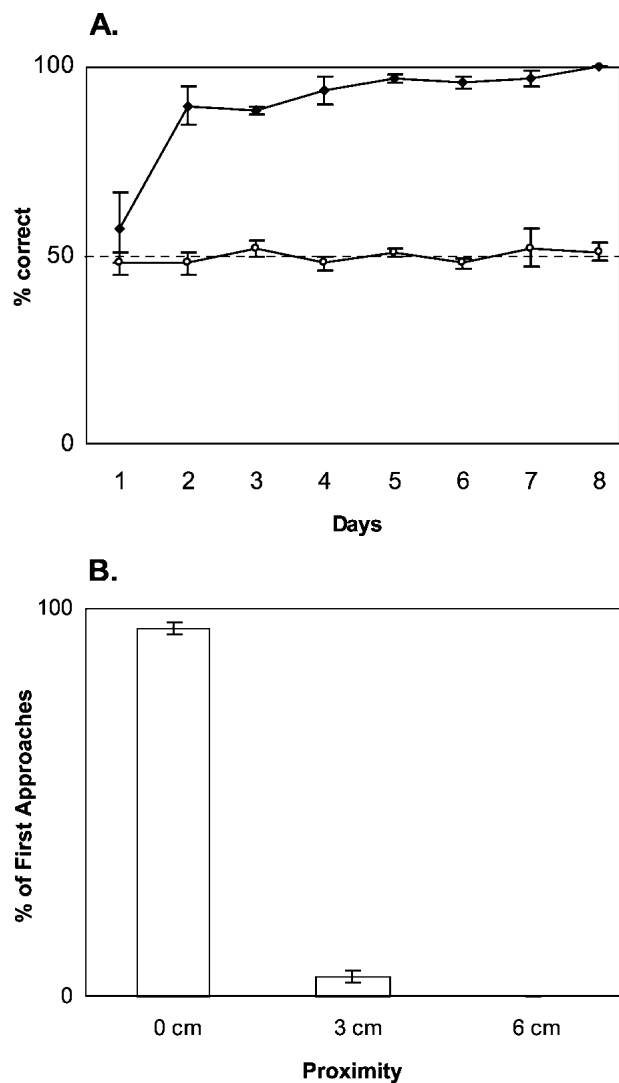
Figure 3 Detection of odors on the platform by normal rats ( n=4 ). (A) First approach (○) and choice (◆) responses (mean \pm SE). Dashed line: chance. (B) Proximity to cups in the first approach (mean \pm SE). 0 cm, rat's nose is over the cup; 3 cm, rat's nose is within 3 cm; 6 cm, rat's nose is within 6 cm.
