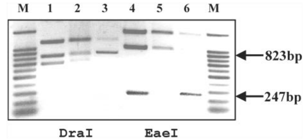
Figure 4. Affinity captures of a specific fragment by biotin-labeled PNA. Lanes 1–3 show fragments with blunt ends obtained by DraI restriction enzyme. Lines 4–6 show fragments with uneven ends obtained by EaeI restriction enzyme. Lanes 1 and 4 show the plasmid fragments after restriction but before capturing. Lanes 2 and 5 and lanes 3 and 6 show non-captured and captured material, respectively. M is a 100 bp dsDNA size marker (Promega).
