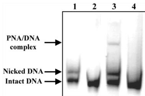
Figure 7. Strand invasion from a single-stranded nick within duplex DNA. Lanes 1 and 3 show the DNA fragments with the nick generated by N.A1wI nicking enzyme. Lines 2 and 4 show intact fragments without a nick. Lanes 3 and 4 show the complex this DNA fragments with PNA 1720. Note that the nicked DNA fragment moves somewhat slower than intact dsDNA (58), thus making it possible to directly monitor further transformations of nicked DNA.
