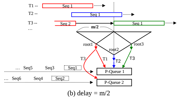
Figure 5. Reducing delay between database sequences
