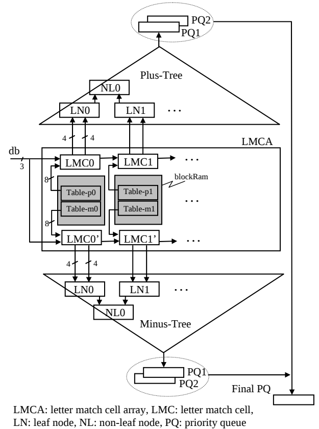
Figure 3. Global view of TreeBLASTn
