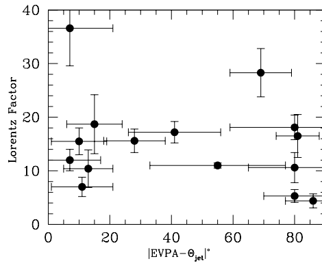
Fig. 4 Lorentz factor vs alignment between EVPA at 7 mm for maximum observed fractional polarization and jet direction.
