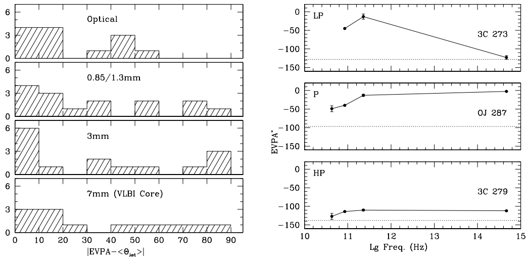
Fig. 3 Left panel: Distributions of the EVPA for maximum observed fractional polarization. Right panel: Dependence of the EVPA on frequency for nearly simultaneous observations (2000 April 3-5); dotted lines show direction of the inner jet.
