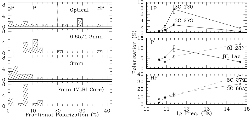
Fig. 1 Left panel: Distributions of maximum observed fractional polarization. Right panel: Examples of dependence of degree of polarization on frequency for nearly simultaneous observations.
