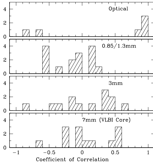
Fig. 2 Distribution of linear correlation coefficients between degree of polarization and total flux.
