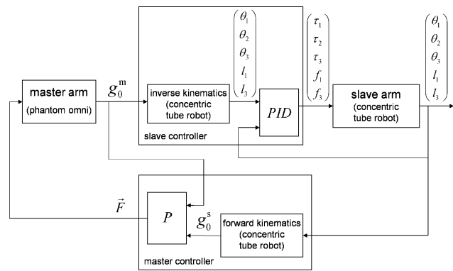
Fig. 19. Teleoperator block diagram.
