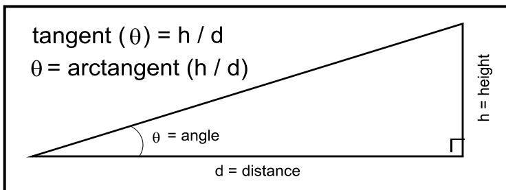
Figure 1: Right triangle showing the relation between the tangent of the opening angle and the ratio of the sides of the triangle.
