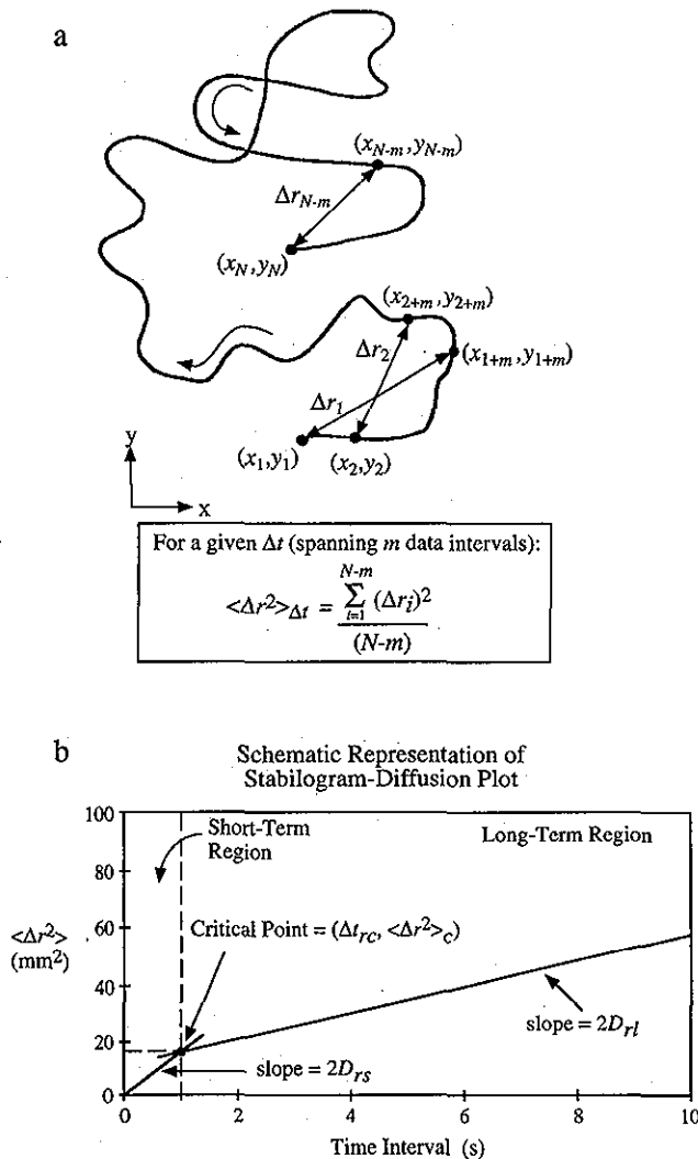
FIG. 2. (a) Diagram showing the method for calculating mean square planar displacement \langle \Delta r^2 \rangle as a function of time interval \Delta t for a COP trajectory made up of N data points (x_1, y_1; x_2, y_2; \dots; x_N, y_N) . In this case, \Delta t does not represent the sampling interval; instead, \Delta t represents a moving time window spanning m data intervals. (b) A schematic representation of a typical resultant planar stabilogram-diffusion plot ( \langle \Delta r^2 \rangle vs \Delta t ) generated from COP time series according to the method shown in (a). The diffusion coefficients D_{rs} and D_{rl} are computed from the slopes of the lines fitted to the short-term and long-term regions, respectively. The critical point, (\Delta t_{rc}, \langle \Delta r^2 \rangle_c) , is defined by the intersection of the lines fitted to the two regions of the plot. The scaling exponents H_{rs} and H_{rl} are calculated from the slopes of the log-log plots of the short-term and long-term regions, respectively (adapted from Collins and De Luca 5 ).
