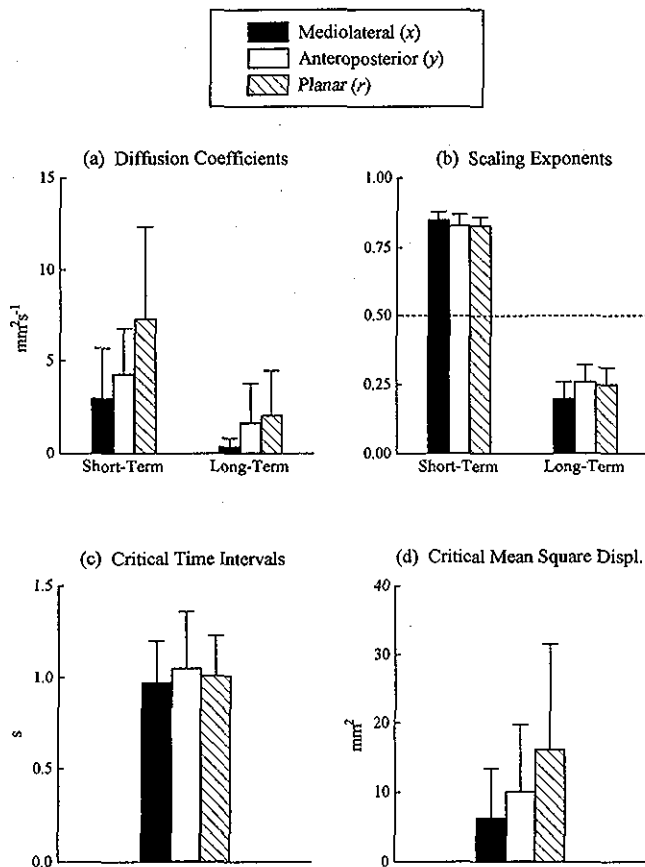
FIG. 4. Group means and standard deviations for the ten subjects: (a) diffusion coefficients, (b) scaling exponents, (c) critical time intervals, and (d) critical mean square displacements. In (b), a dashed line is drawn at the value expected for classical Brownian motion, i.e., H_{ii}=0.50 .
