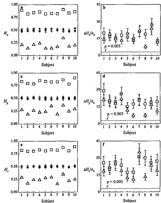
FIG. 5. Random-walk analyses of COP time series and shuffled surrogate data sets. (a) Calculated values of H_x for the short-term ( \square ) and long-term ( \Delta ) scaling regions of the original COP time series and for the shuffled surrogates ( + ) for each of the ten subjects. (b) The significance of the differences between the computed H_x values for the original COP time series and the surrogates in (a). The significance values and error bars were calculated according to the techniques described by Theiler et al. 17 Here \sigma_x is the standard deviation of the H_x values for the surrogates, and \Delta H_x is the difference between the value of H_x for the original COP time series and the mean value of H_x for the surrogates. A dashed line is plotted at the significance level that corresponds to a p value of 0.005. (c) As in (a), but for the anteroposterior scaling exponents ( H_y ). (d) As in (b), but for the computed values of H_y in (c). (e) As in (a), but for the planar scaling exponents ( H_r ). (f) As in (b), but for the computed values of H_r in (e).
