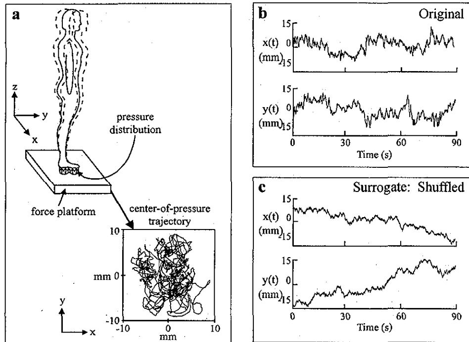
FIG. 1. (a) A schematic diagram of the experimental setup for examining quiet-standing postural stability. Shown also is a typical 90 s stabilogram for a healthy young individual. (b) The x -coordinate and y -coordinate time series corresponding to the stabilogram in (a). (c) Shuffled surrogate random-walk data sets that were generated from the original COP time series in (b).
