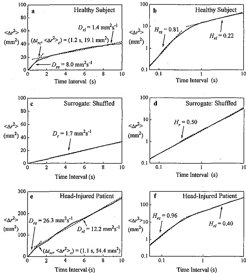
FIG. 3. Resultant (a) linear-linear and (b) log-log plots of mean square planar COP displacement versus time interval for a representative subject. Also shown in (a) and (b) are the fitted regression lines (dashed lines) for the short-term and long-term regions and the computed values for the respective stabilogram-diffusion parameters. (c) As in (a), but for shuffled surrogate random-walk data sets that were generated from the original COP time series. (d) As in (b), but for the surrogates in (c). (e) As in (a), but for a patient with a mild head injury. (f) As in (b), but for the patient in (e).
